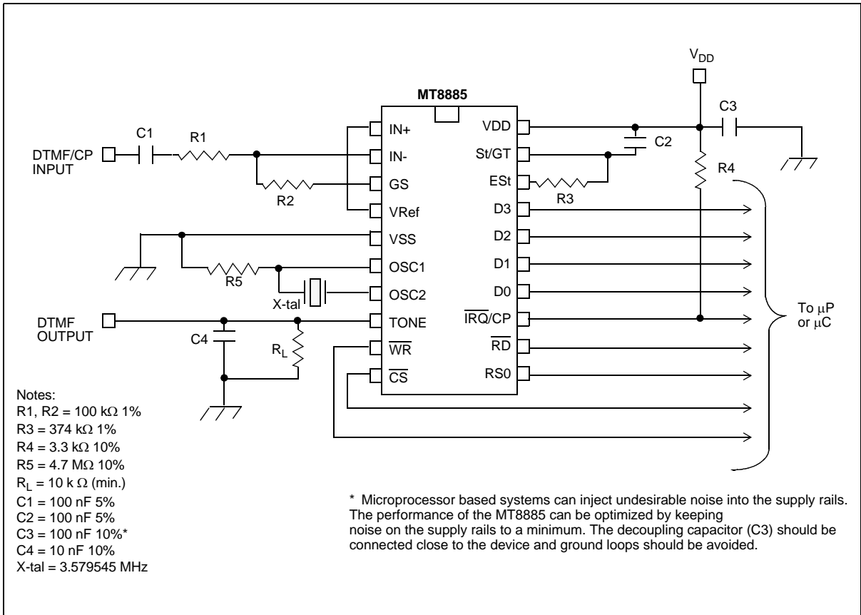
Figure 13 - Application Circuit (Single-Ended Input)
