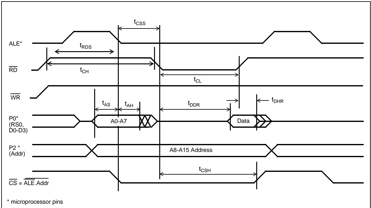
Figure 17 - Intel Read Timing Diagram
