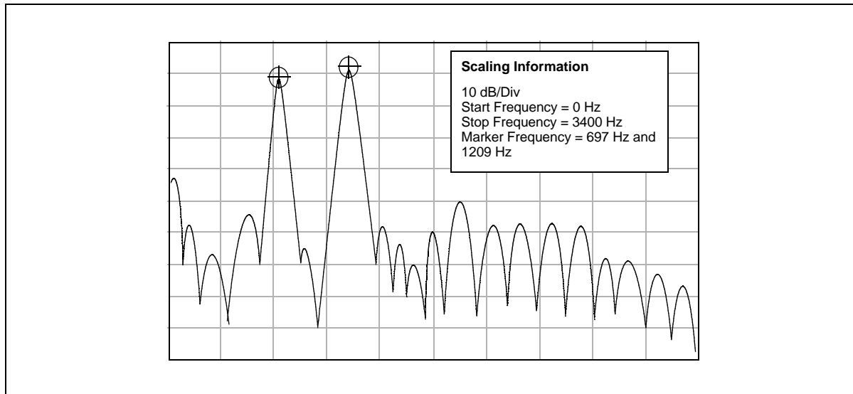
Figure 10 - Spectrum Plot
