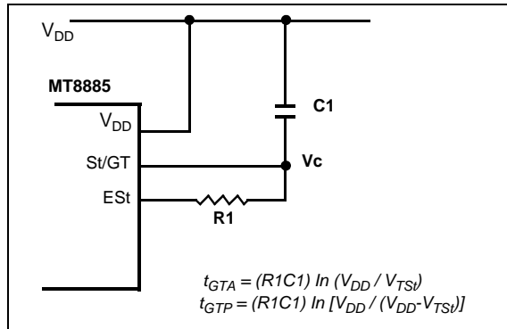
Figure 5 - Basic Steering Circuit
