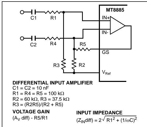
Figure 4 - Differential Input Configuration
