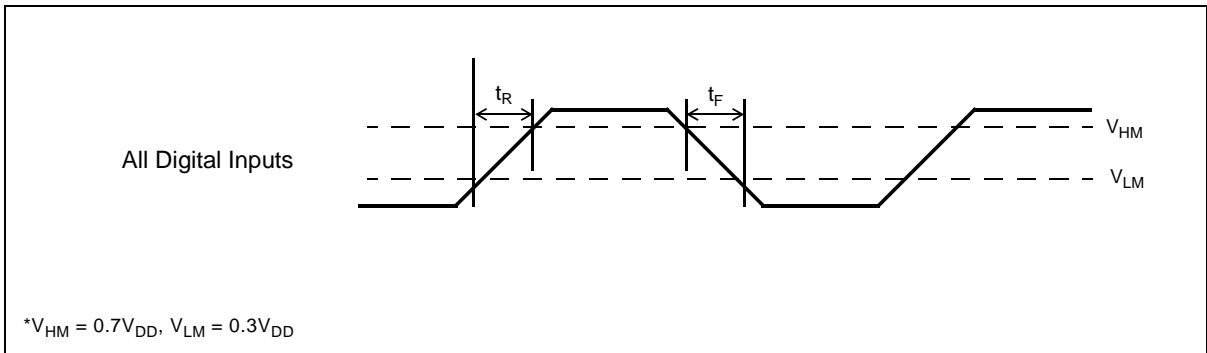
Figure 15 - Digital Signal Input Rise/Fall Times
