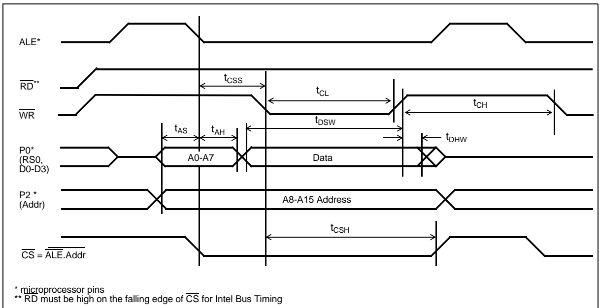
Figure 18 - Intel Write Timing Diagram
