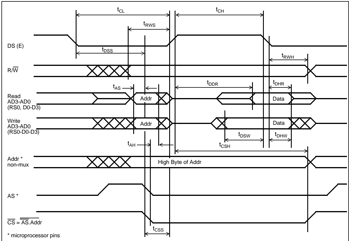
Figure 16 - Motorola BUS Timing Diagram
