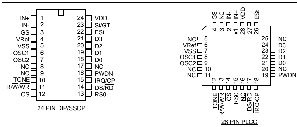
Figure 2 - Pin Connections
